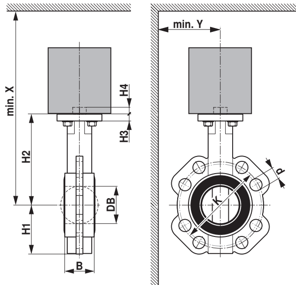
Dimensional drawings
